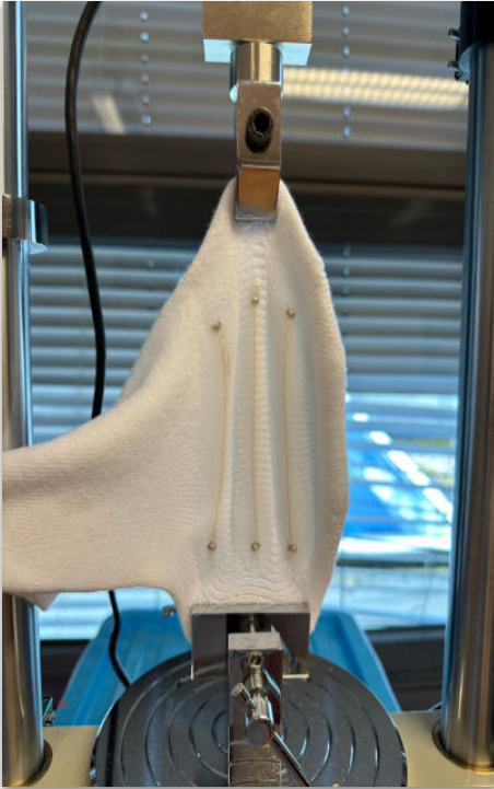
sendance-grid testing
